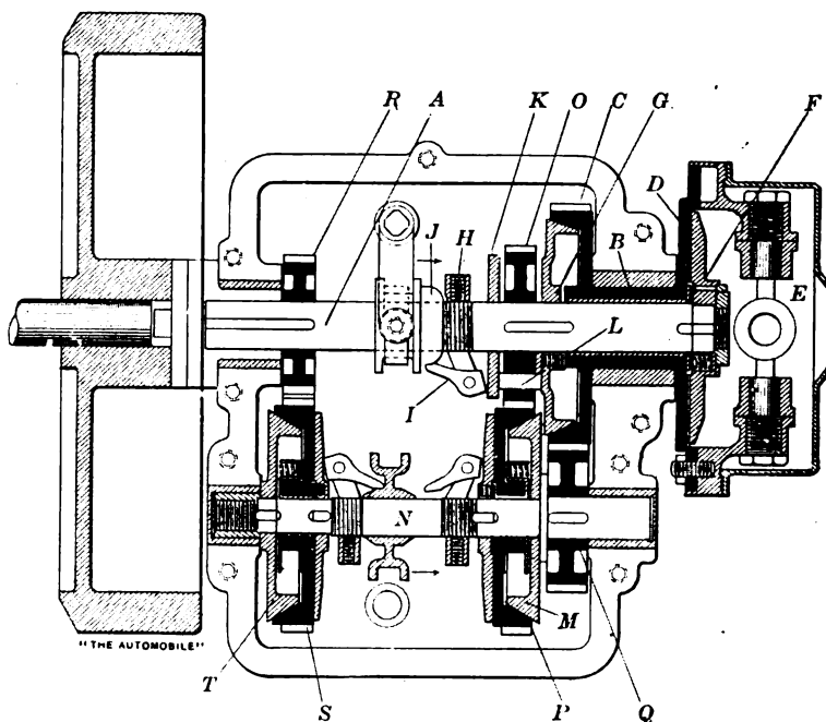
FIG. 1.—SECTIONAL DRAWING OF WINTON INDIVIDUAL CLUTCH SYSTEM.
